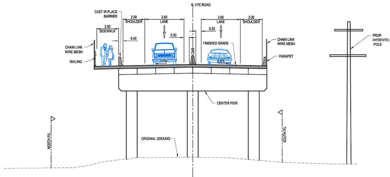
VYE ROAD OVERPASS - TYPICAL SECTION (LOOKING EAST) SCALE 1:100
