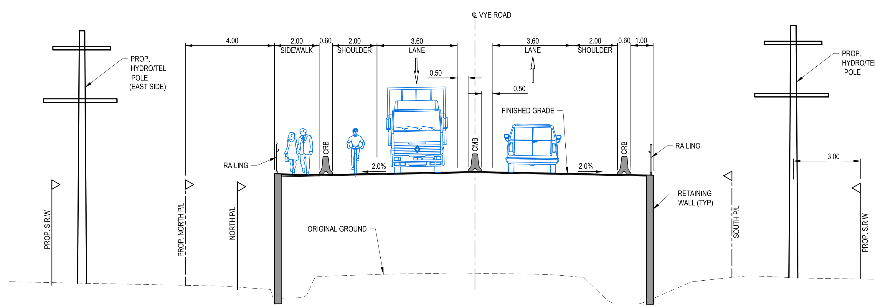
VYE ROAD - TYPICAL SECTION WITH WALL (LOOKING EAST) SCALE 1:100
