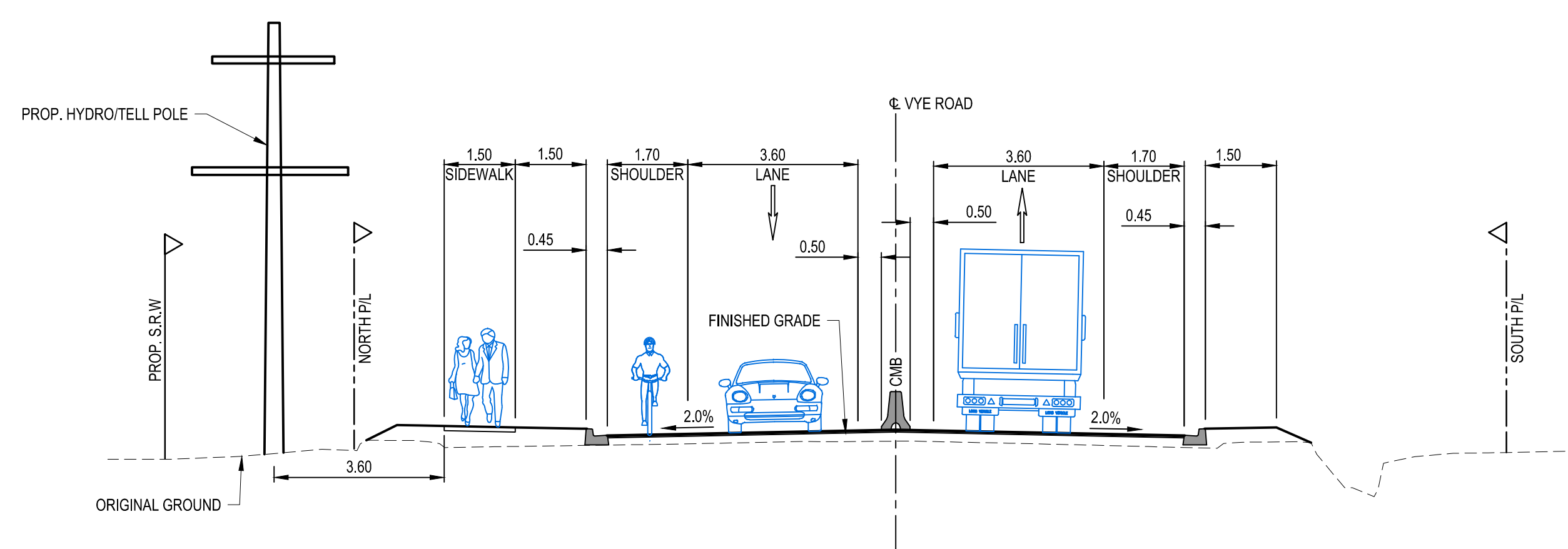
VYE ROAD - TYPICAL SECTION (LOOKING EAST) SCALE 1:100
