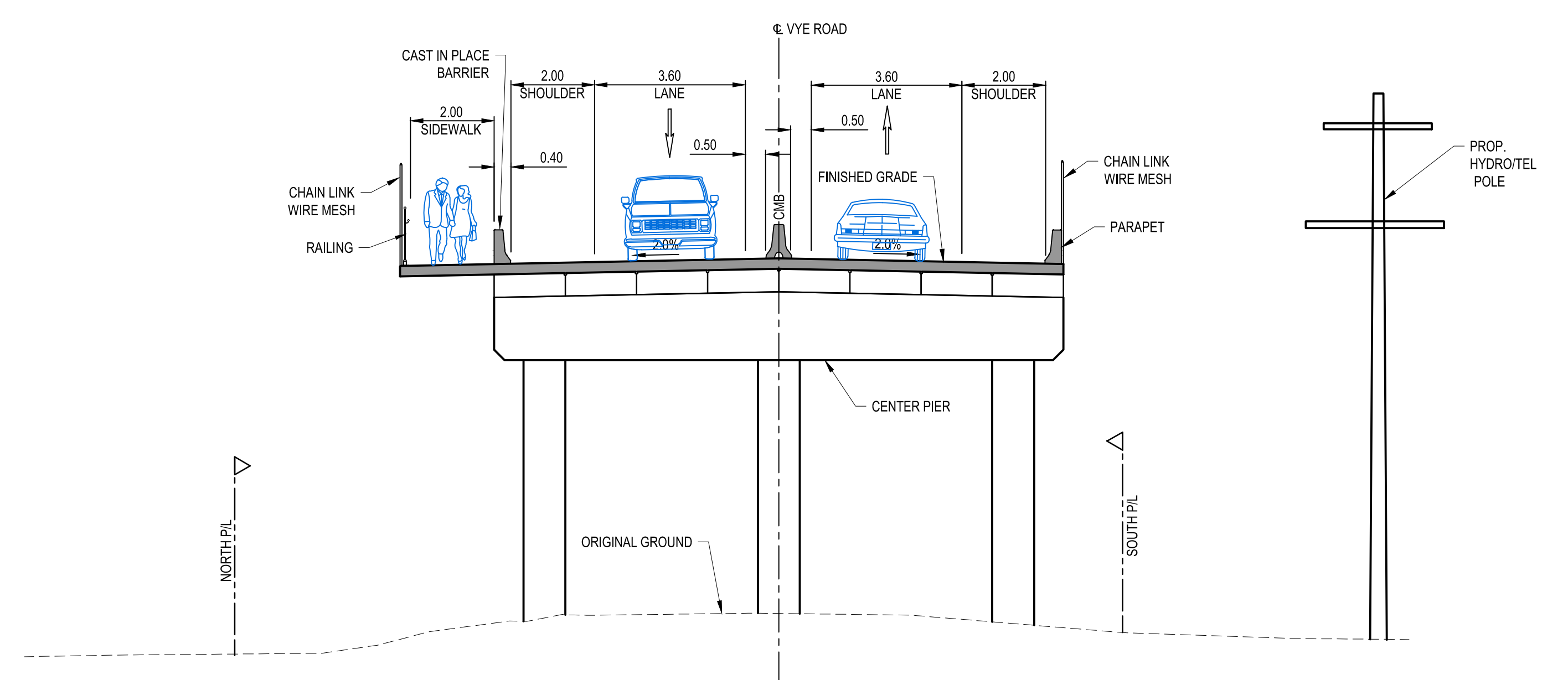
VYE ROAD OVERPASS - TYPICAL SECTION (LOOKING EAST) SCALE 1:100
